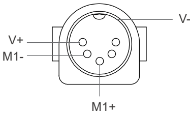
Moteck U-type 5-pin DIN male plug (Moteck pinout: C-DIN-51H)
