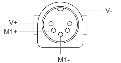
Moteck U-type 5-pin DIN male plug
