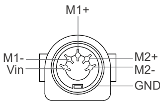
Moteck U-type 5-pin DIN male plug (Moteck pinout: C-DIN-52H)
