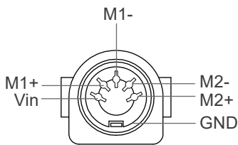
Moteck U-type 5-pin DIN male plug (Moteck pinout: C-DIN-52R)
